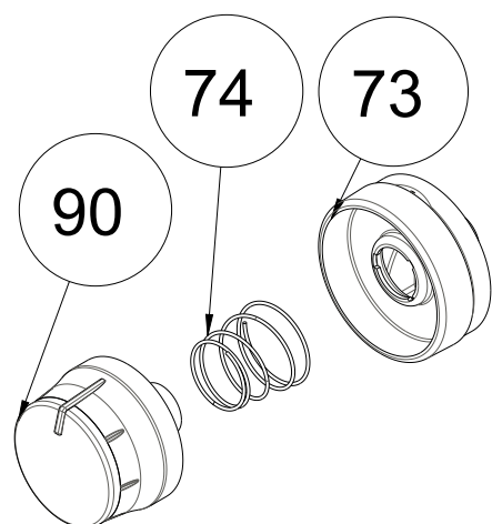
SPECTRUM
